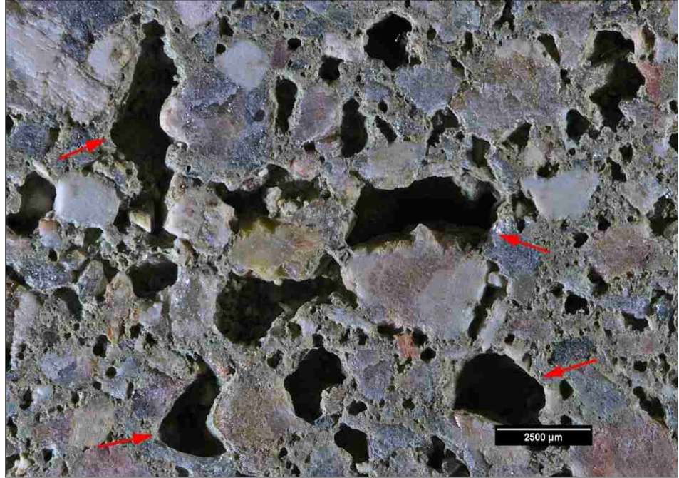
Figure 14. Entrapped voids (Source DRP)
