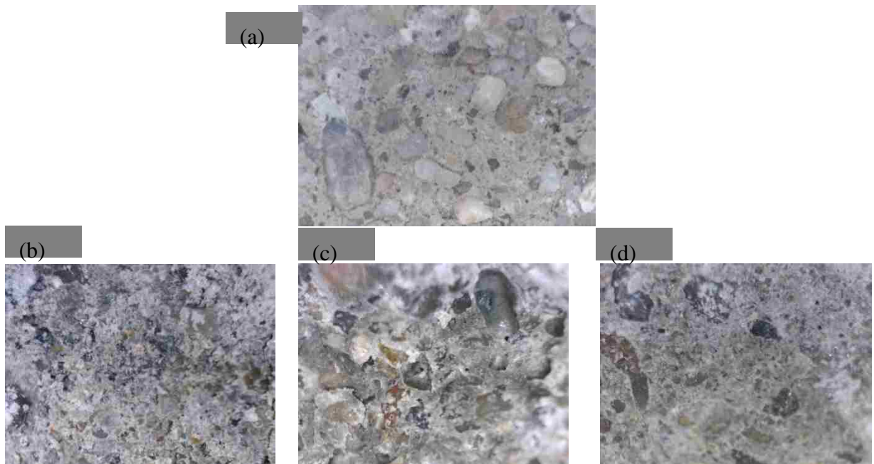
Figure 11. Digital microscope; (a) historical surface; (b) batch #1; (c) batch #2; (d) batch #3.
