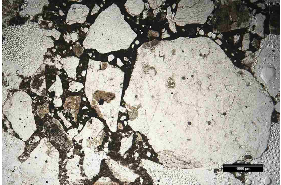
Figure 7. Petrographic analysis in plane-polarization (Source: DRP).
