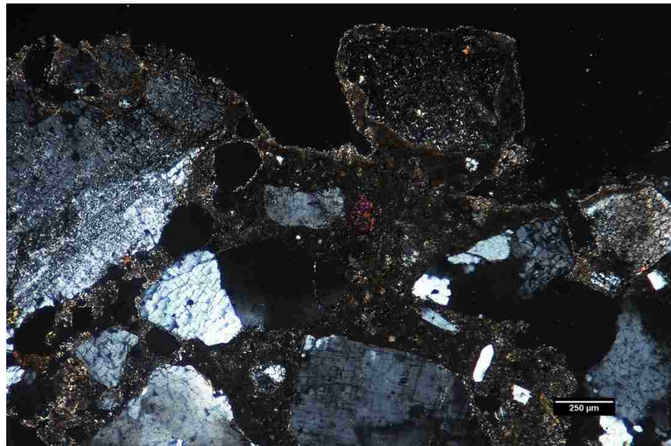
Figure 15. Aged and weathered Portland cement paste (Source: DRP).
