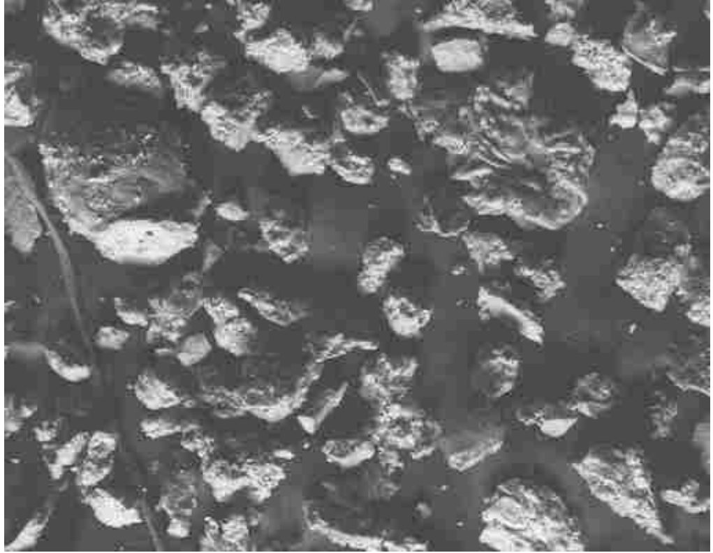
Figure 6. SEM image of historic concrete surface (Source Dr. Brearley).
